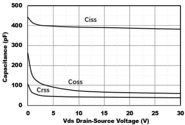
Figure3. Capacitance Characteristics
