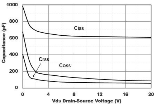
Figure3. Capacitance Characteristics
