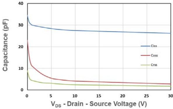
Figure 7. Capacitance
