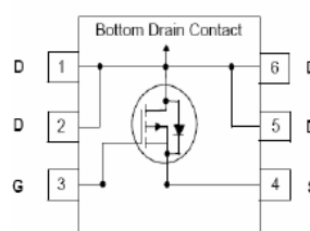
Pin assignment
